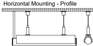
Horizontal Mounting - Profile
